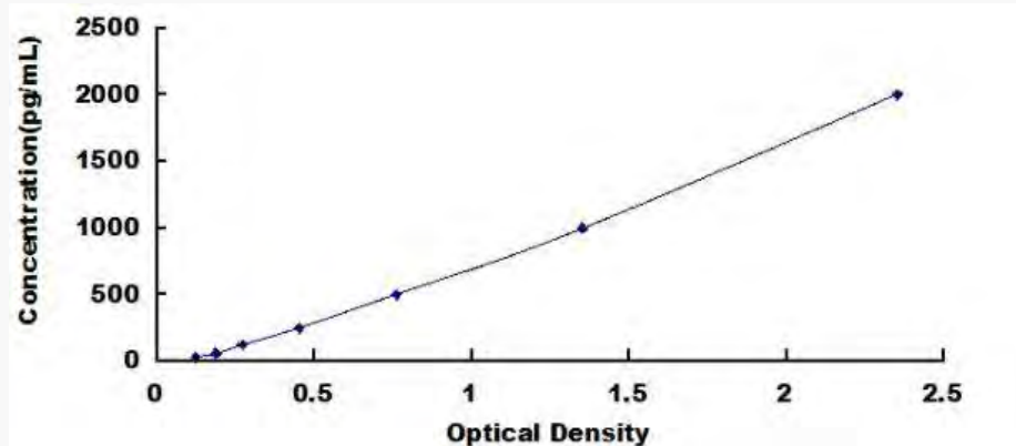
Typical Standard Curve for Human NKCC2 ELISA.
