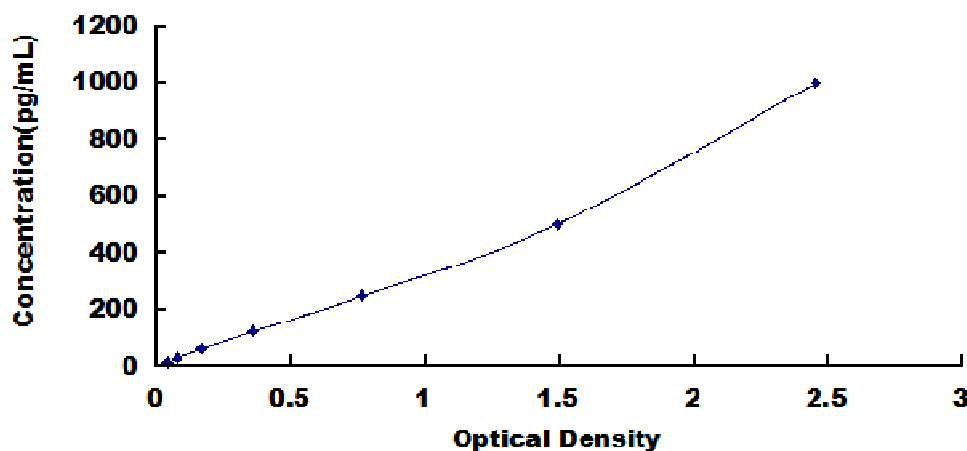
Typical Standard Curve for BMP1, Human ELISA.
