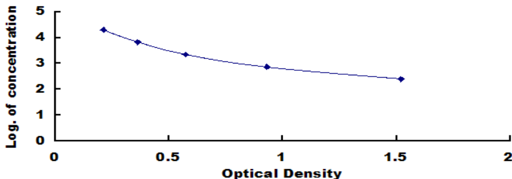
Typical Standard Curve for MOTS-c, Mouse ELISA.
