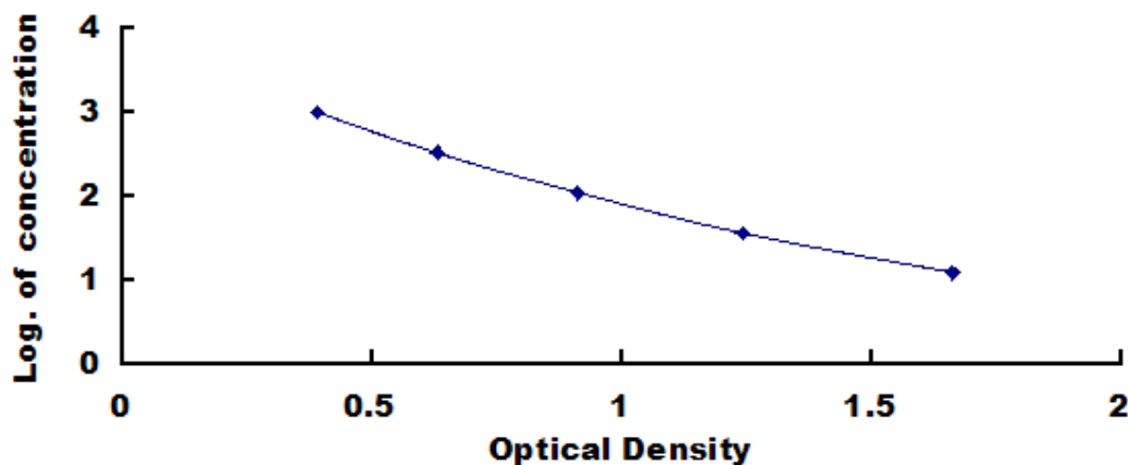
Typical Standard Curve for BNP, Gallus ELISA.
