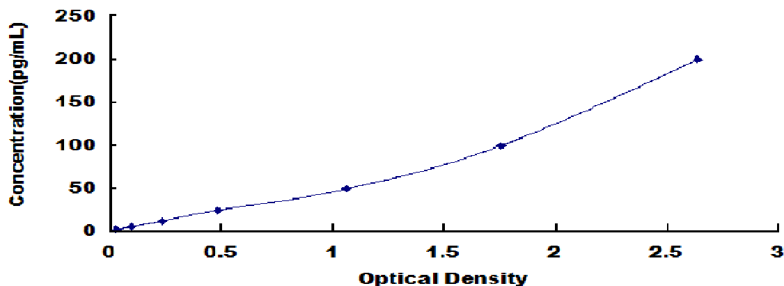
Typical Standard Curve for OC, Gallus ELISA.
